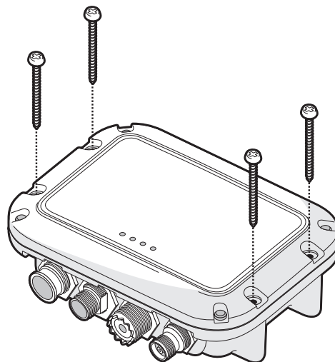
Figure 6 AIS transceiver mounting
