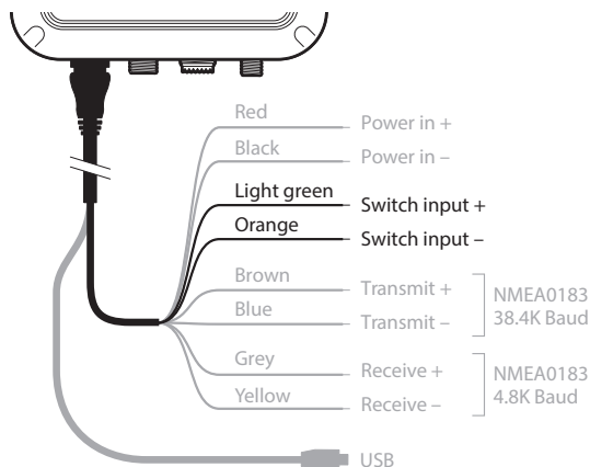
Figure 10 Connecting an external switch
