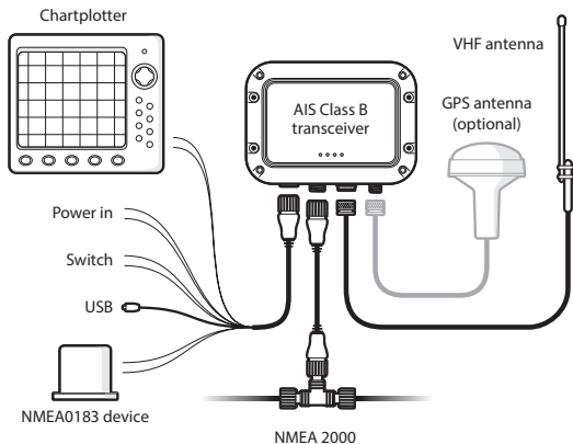
Figure 4 Typical installation configuration
