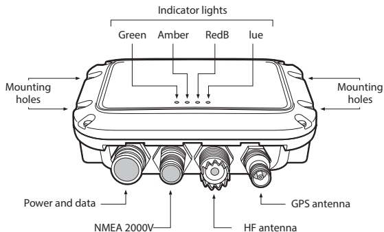
Figure 2 AIS transceiver overview
