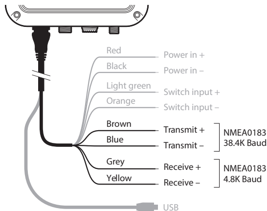
Figure 11 Connecting to the NMEA0183 data port.
