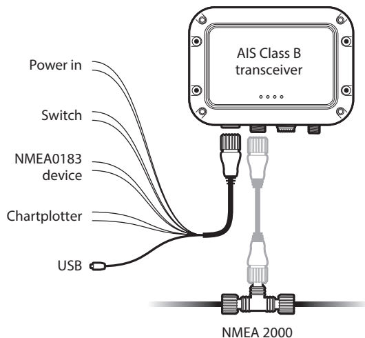
Figure 3 Electrical connections to the AIS transceiver
