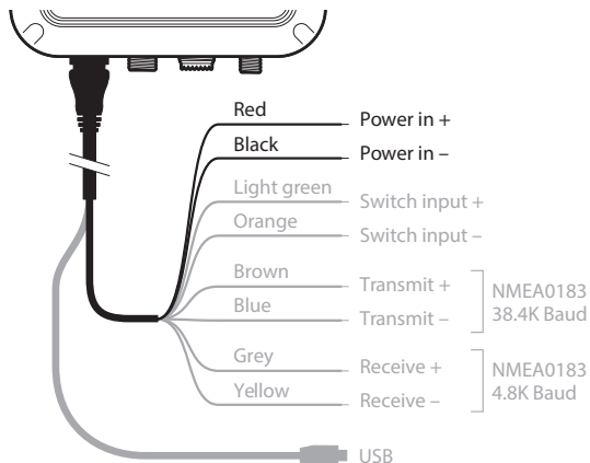
Figure 12 Connecting the power supply
