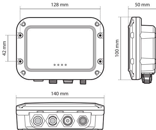
Figure 5 AIS transceiver dimensions
