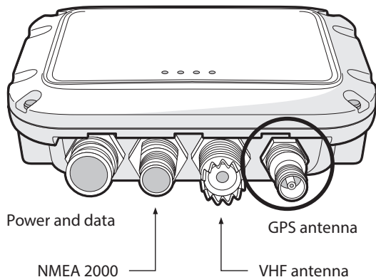
Figure 8 Position of the GPS antenna connector
